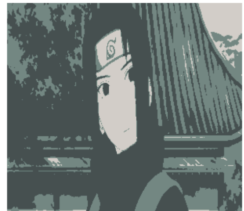
K-Means
