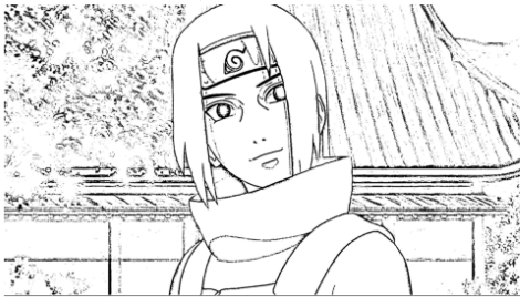
Adaptive Thresholding
